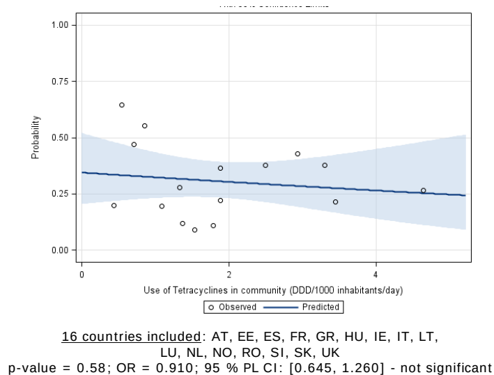
Figure 32. Logistic regression analysis curves with OR estimates and 95 % PL CIs of the national consumption of tetracyclines in the community in humans and the probability of clinical resistance to tetracycline in Salmonella spp. from human infections for the year 2012—dots represent the countries involved in the analysis
